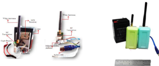
Gambar 4. Hasil Rangkaian Prototipe Figure 4 Prototype Circuit Results
