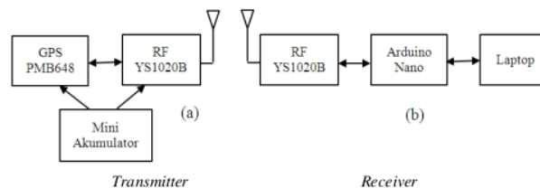
Gambar 1. Konstruksi hardware Figure 1. Hardware construction
